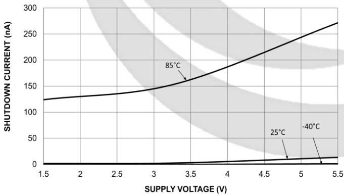
Figure 8. Shutdown Current vs. Input Voltage
