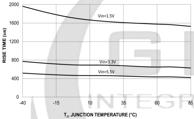
Figure 12. V_{OUT} Rise Time vs. Temperature
