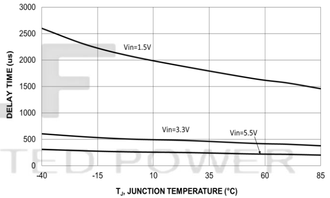
Figure 13. Turn-On Delay Time vs. Temperature
