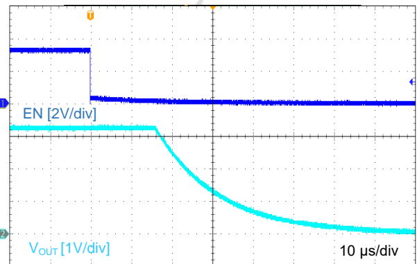
Figure 15. Turn-Off Response, GLF1110 V_{IN}=3.3\text{ V} , C_{IN}=0.1\text{ }\mu\text{F} , C_{OUT}=0.1\text{ }\mu\text{F} , R_L=150\text{ }\Omega
