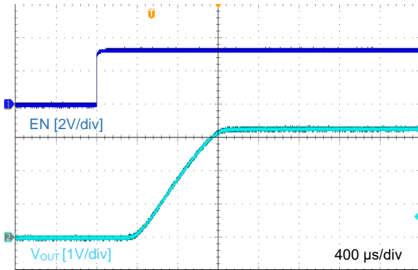
Figure 16. Turn-On Response, GLF1111 V_{IN}=3.3\text{ V} , C_{IN}=0.1\text{ }\mu\text{F} , C_{OUT}=0.1\text{ }\mu\text{F} , R_L=150\text{ }\Omega
