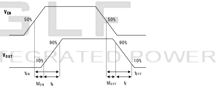
Figure 3. Timing Diagram
