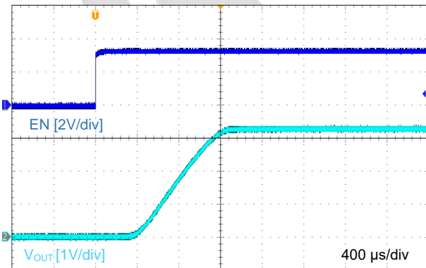
Figure 14. Turn-On Response, GLF1110 V_{IN}=3.3\text{ V} , C_{IN}=0.1\text{ }\mu\text{F} , C_{OUT}=0.1\text{ }\mu\text{F} , R_L=150\text{ }\Omega
