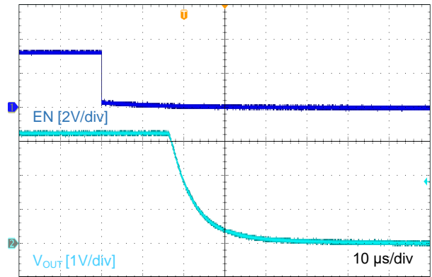
Figure 17. Turn-Off Response, GLF1111 V_{IN}=3.3\text{ V} , C_{IN}=0.1\text{ }\mu\text{F} , C_{OUT}=0.1\text{ }\mu\text{F} , R_L=150\text{ }\Omega
