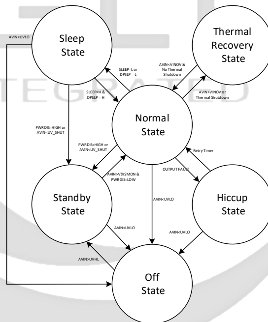
Figure 4. State Machine
