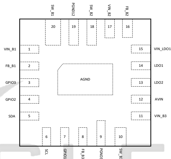
Figure 2. Pin Configuration
