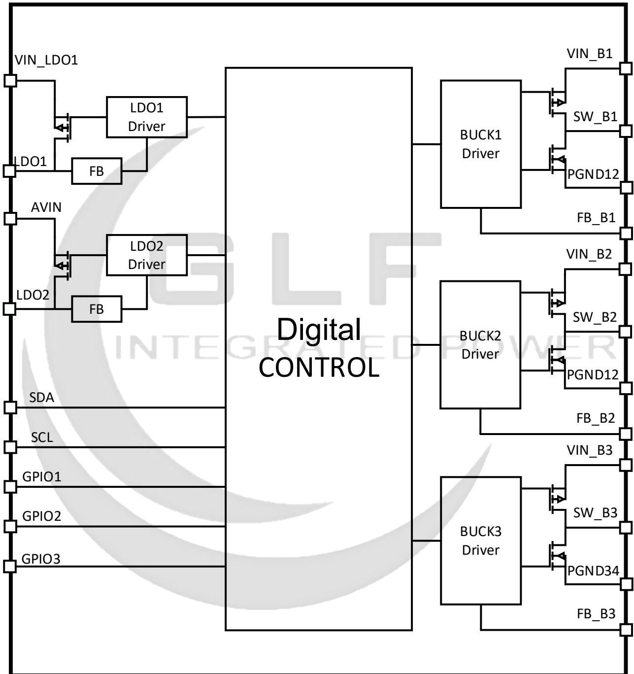
Figure 3. Block Diagram
