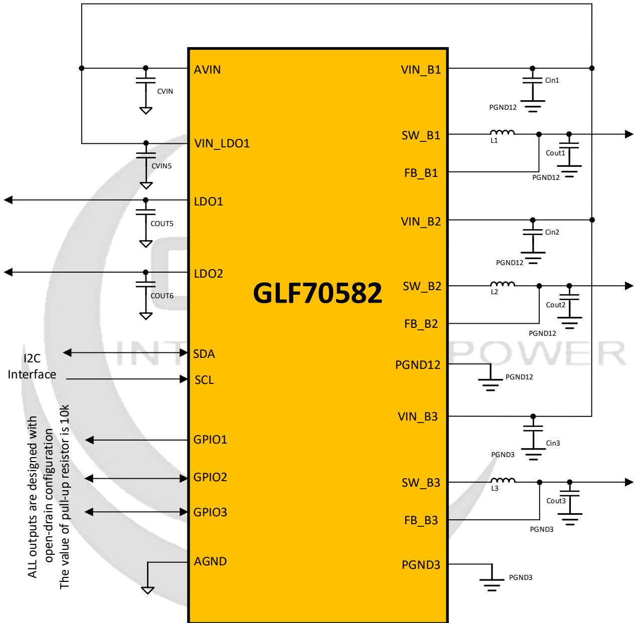
Figure 5. System Example
