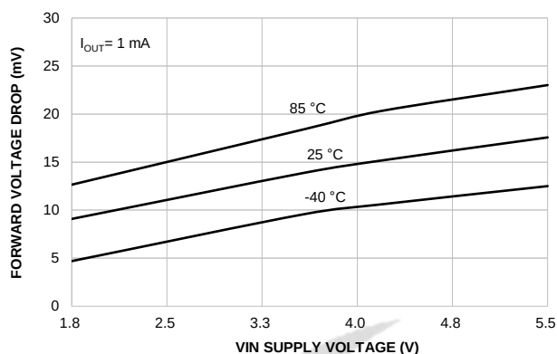
Figure 15. Forward Voltage Drop vs. Supply Voltage (Low Output Current, GLF1800 and GLF1800A)
