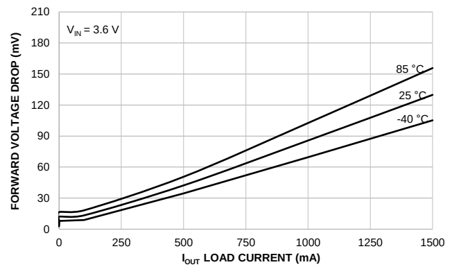
Figure 10. Forward Voltage Drop vs. Load Current, GLF1800T and GLF1800AT
