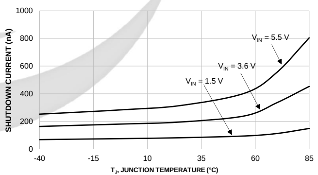
Figure 8. Shutdown Current vs. Temperature GLF1800A and GLF1800AT
