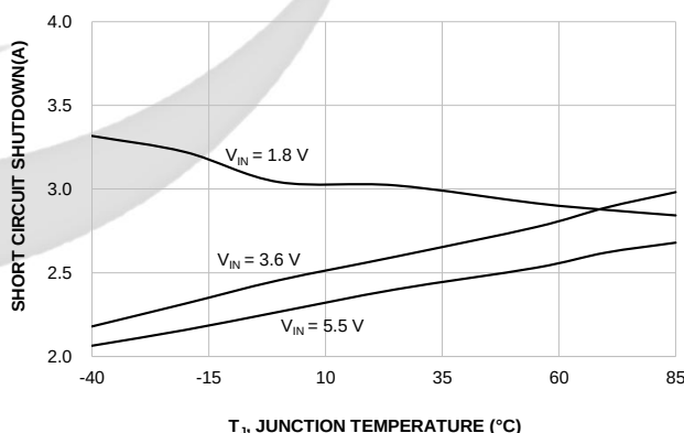
Figure 20. Short Circuit Current vs. Temperature, GLF1800T and GLF1800AT
