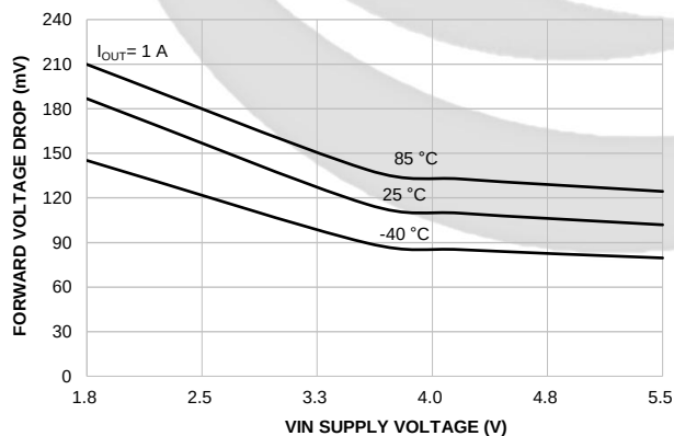
Figure 13. Forward Voltage Drop vs. Supply Voltage (High Output Current, GLF1800 and GLF1800A)
