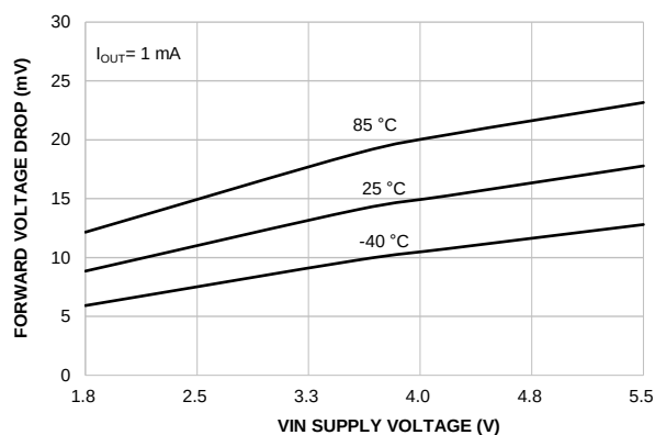
Figure 16. Forward Voltage Drop vs. Supply Voltage (Low Output Current, GLF1800T and GLF1800AT)
