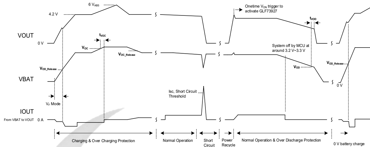
Figure 2. Operation Diagram
