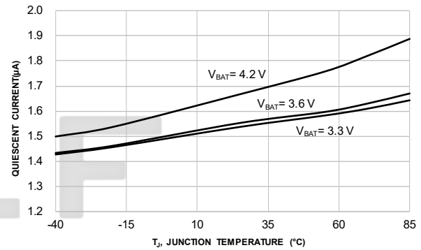
Figure 15. Quiescent Current vs. Temperature
