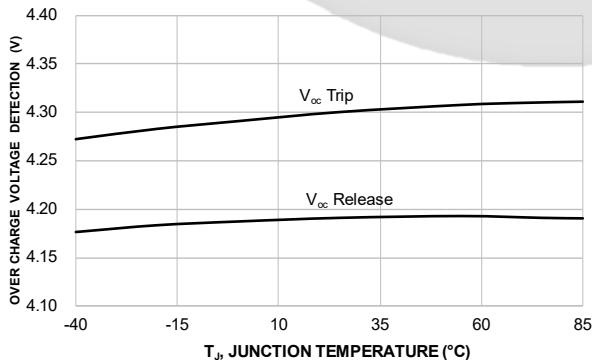
Figure 10. GLF73927C Over Charge Voltage Detection vs. Temperature
