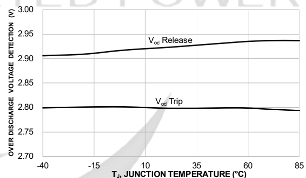
Figure 9. GLF73927B Over Discharge Voltage Detection vs. Temperature
