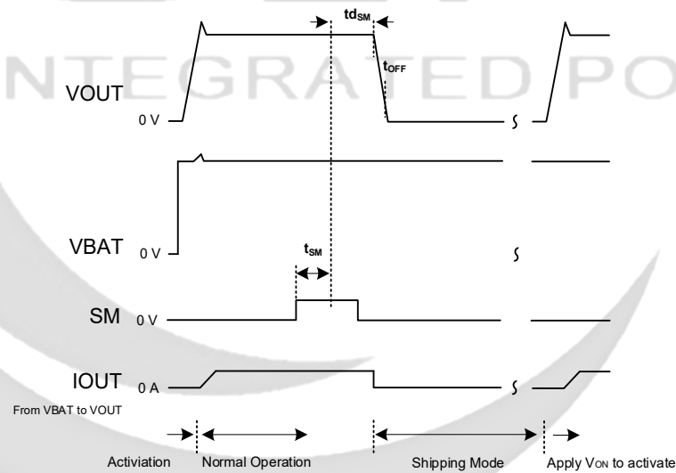
Figure 3. Shipping Mode Operation
