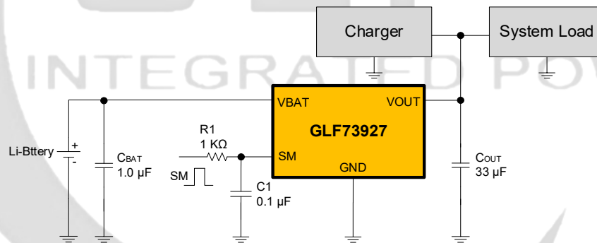
Figure 1. Application Diagram
