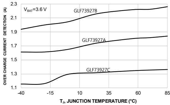
Figure 12. Over Charge Current Protection vs. Temperature
