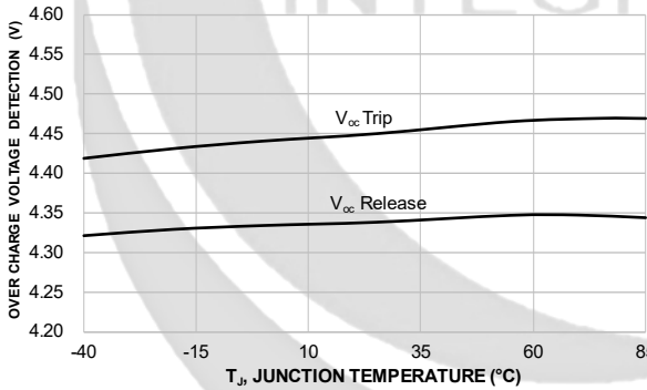
Figure 8. GLF73927B Over Charge Voltage Detection vs. Temperature
