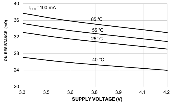
Figure 13. On-Resistance vs. Supply Voltage
