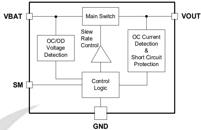
Figure 4. Functional Block Diagram
