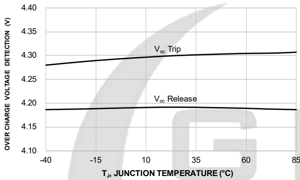
Figure 6. GLF73927A Over Charge Voltage Detection vs. Temperature
