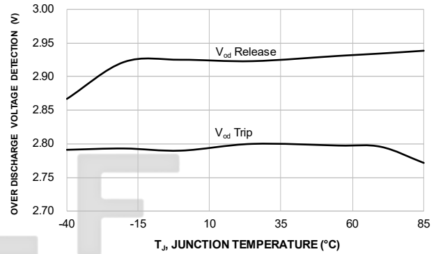
Figure 7. GLF73927A Over Discharge Voltage Detection vs. Temperature
