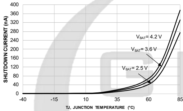
Figure 14. Shutdown Current vs. Temperature
