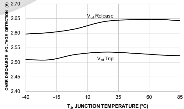
Figure 11. GLF73927C Over Discharge Voltage Detection vs. Temperature
