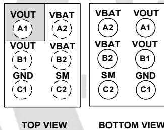
Figure 5. 0.97mm x 1.47mm x 0.55mm WLCSP
