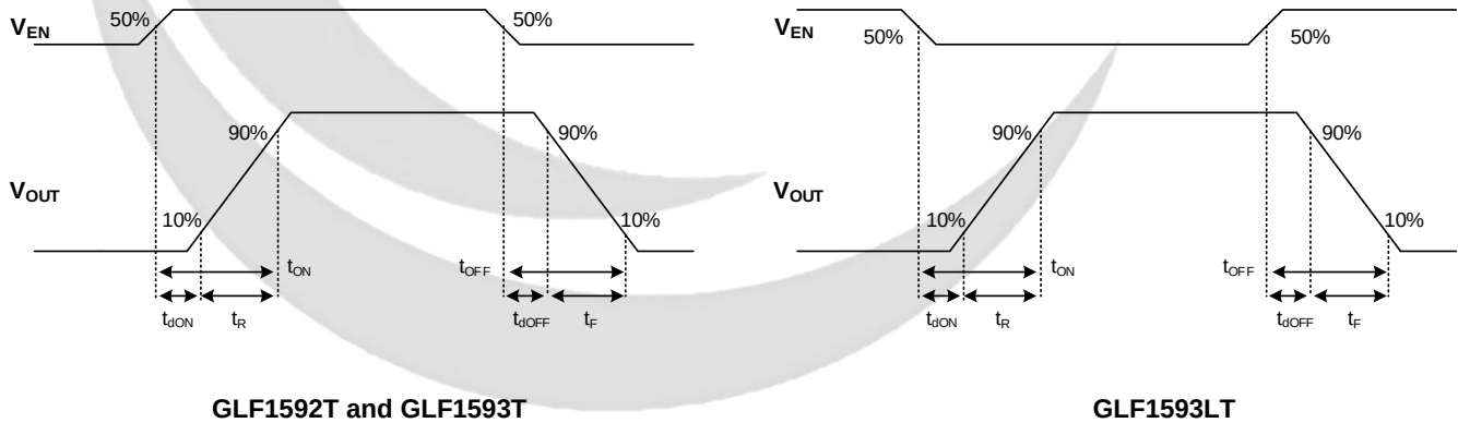
Figure 4. Timing Diagram
