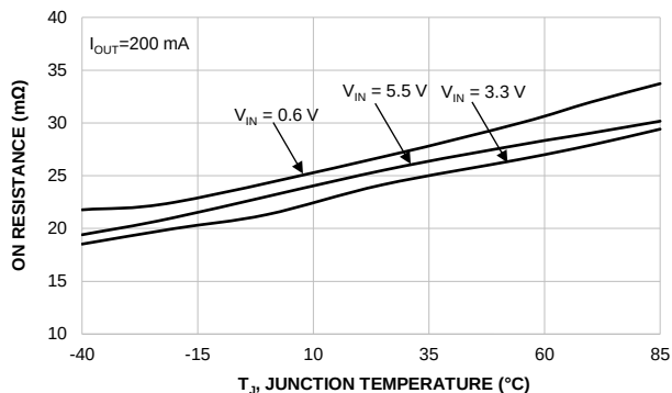
Figure 6. On-Resistance vs. Temperature
