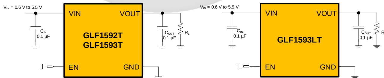
Figure 1. Application diagram
