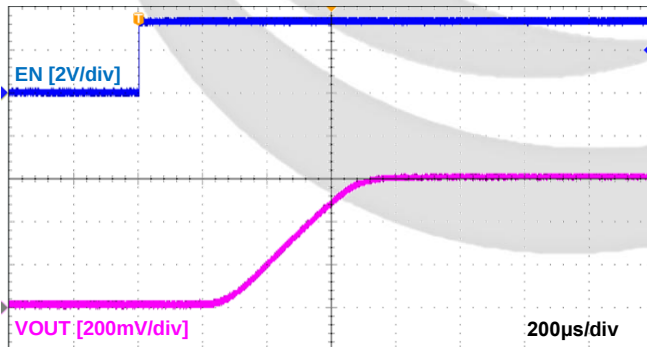
Figure 15. Turn-On Response V_{IN}=0.6\text{ V} , V_{EN}=3.3\text{ V} , C_{OUT}=0.1\text{ }\mu\text{F} , R_L=150\text{ }\Omega , GLF1593T
