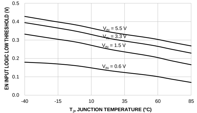
Figure 12. EN Input Logic Low Threshold vs. Temperature
