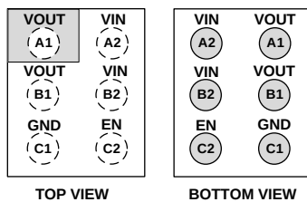
Figure 3. 0.67 mm x 1.02 mm x 0.35 mm Thin WLCSP
