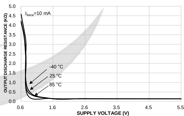
Figure 10. Output Discharge Resistance vs. Supply Voltage
