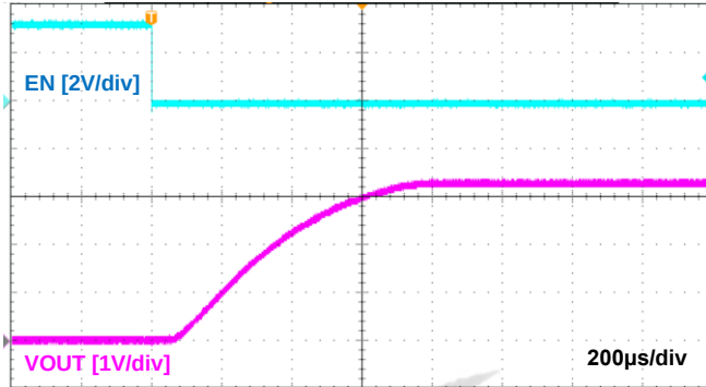
Figure 17. Turn-On Response V_{IN}=V_{EN}=3.3\text{ V} , C_{OUT}=0.1\text{ }\mu\text{F} , R_L=150\text{ }\Omega , GLF1593LT
