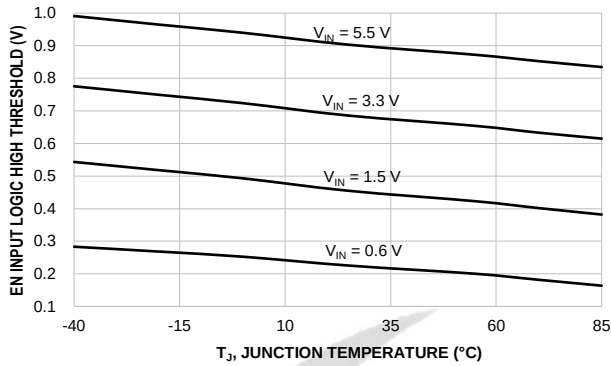
Figure 11. EN Input Logic High Threshold vs. Temperature
