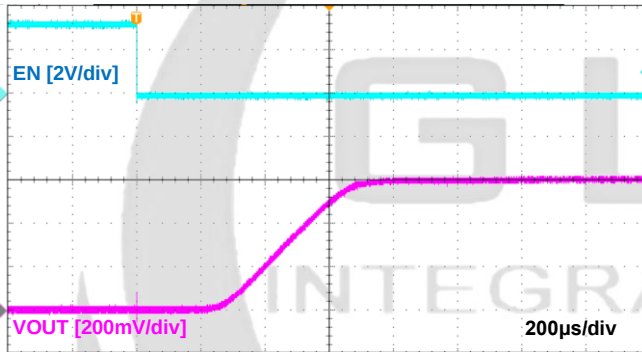
Figure 19. Turn-On Response V_{IN}=0.6\text{ V} , V_{EN}=3.3\text{ V} , C_{OUT}=0.1\text{ }\mu\text{F} , R_L=150\text{ }\Omega , GLF1593LT
