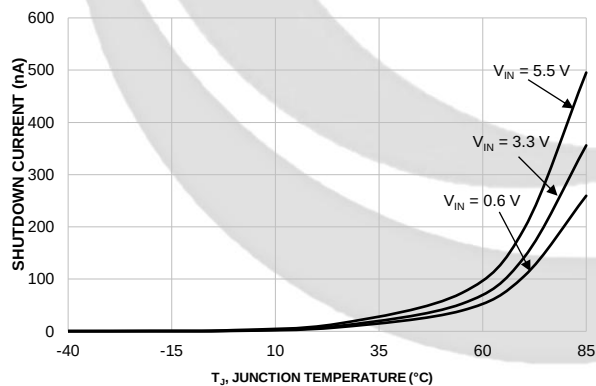
Figure 9. V_{IN} Shutdown Current vs. vs. Temperature
