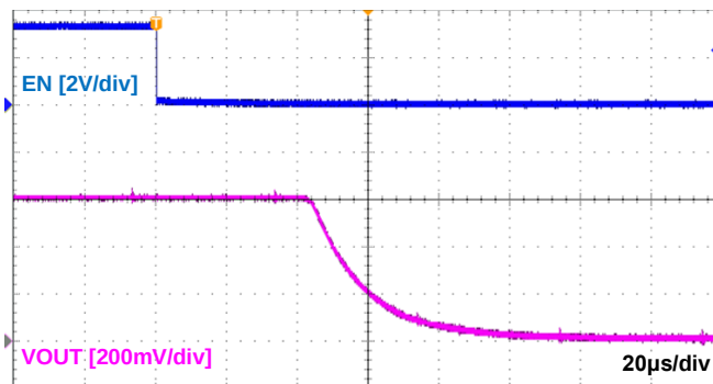
Figure 24. Turn-Off Response V_{IN}=0.6\text{ V} , V_{EN}=3.3\text{ V} , C_{OUT}=0.1\text{ }\mu\text{F} , R_L=150\text{ }\Omega , GLF1592T
