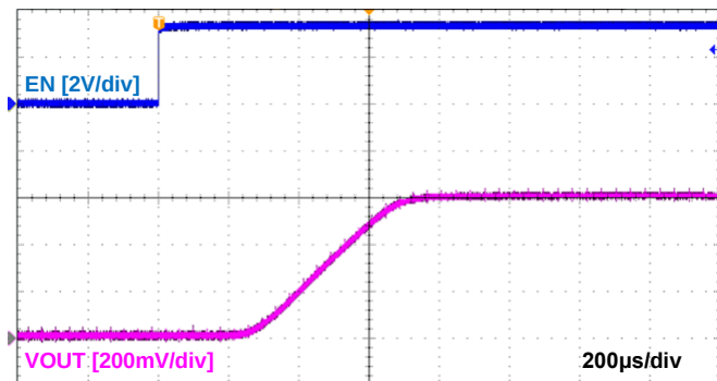
Figure 23. Turn-On Response V_{IN}=0.6\text{ V} , V_{EN}=3.3\text{ V} , C_{OUT}=0.1\text{ }\mu\text{F} , R_L=150\text{ }\Omega , GLF1592T
