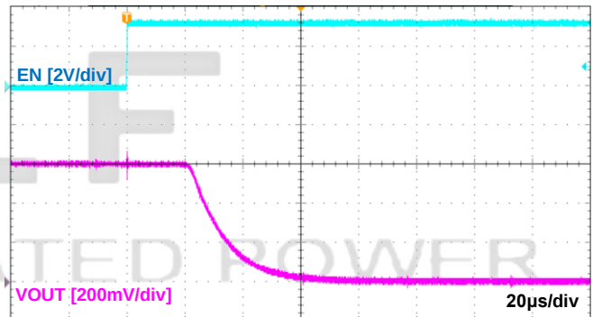
Figure 20. Turn-Off Response V_{IN}=0.6\text{ V} , V_{EN}=3.3\text{ V} , C_{OUT}=0.1\text{ }\mu\text{F} , R_L=150\text{ }\Omega , GLF1593LT
