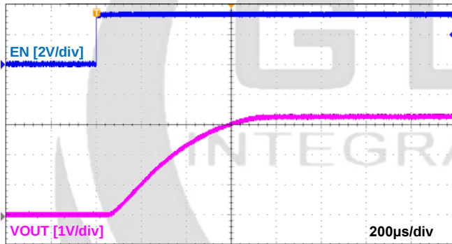
Figure 13. Turn-On Response V_{IN}=V_{EN}=3.3\text{ V} , C_{OUT}=0.1\text{ }\mu\text{F} , R_L=150\text{ }\Omega , GLF1593T
