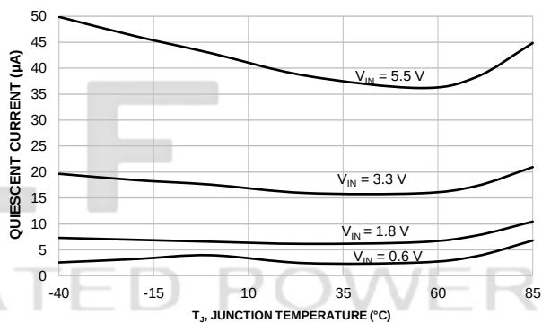
Figure 8. Quiescent Current vs. Temperature
