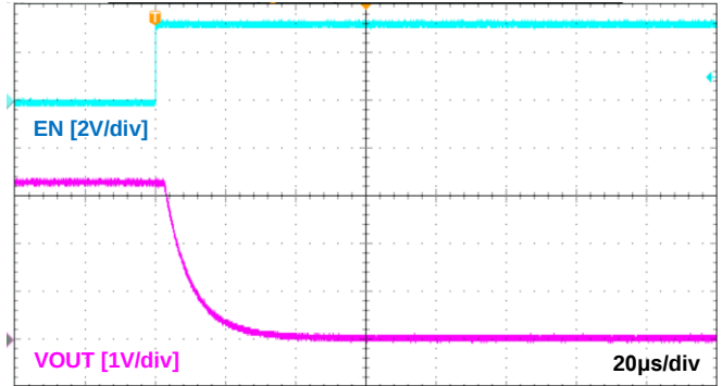
Figure 18. Turn-Off Response V_{IN}=V_{EN}=3.3\text{ V} , C_{OUT}=0.1\text{ }\mu\text{F} , R_L=150\text{ }\Omega , GLF1593LT
