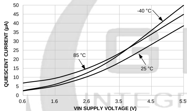
Figure 7. Quiescent Current vs. Supply Voltage
