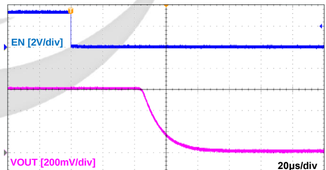
Figure 16. Turn-Off Response V_{IN}=0.6\text{ V} , V_{EN}=3.3\text{ V} , C_{OUT}=0.1\text{ }\mu\text{F} , R_L=150\text{ }\Omega , GLF1593T
