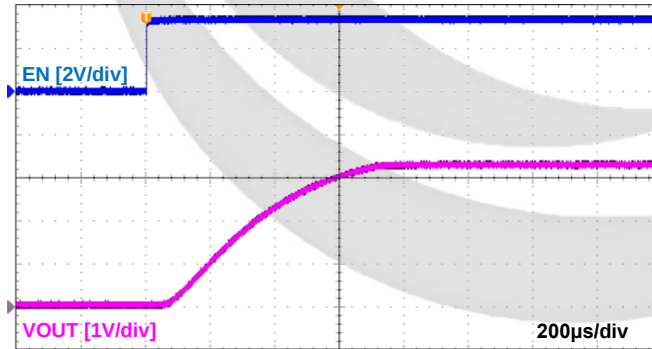
Figure 21. Turn-On Response V_{IN}=V_{EN}=3.3\text{ V} , C_{OUT}=0.1\text{ }\mu\text{F} , R_L=150\text{ }\Omega , GLF1592T
