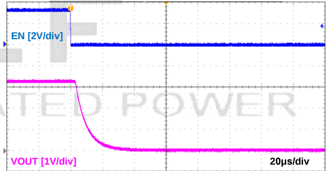
Figure 14. Turn-Off Response V_{IN}=V_{EN}=3.3\text{ V} , C_{OUT}=0.1\text{ }\mu\text{F} , R_L=150\text{ }\Omega , GLF1593T
