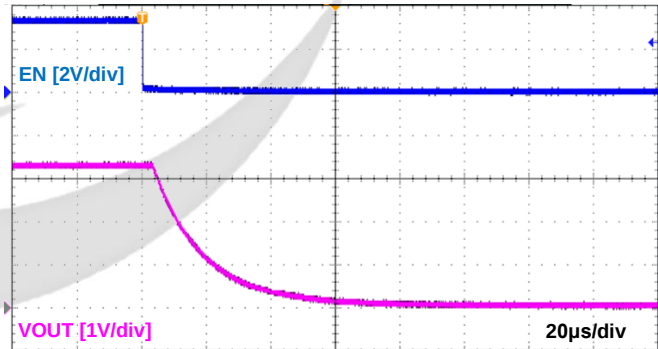
Figure 22. Turn-Off Response V_{IN}=V_{EN}=3.3\text{ V} , C_{OUT}=0.1\text{ }\mu\text{F} , R_L=150\text{ }\Omega , GLF1592T
